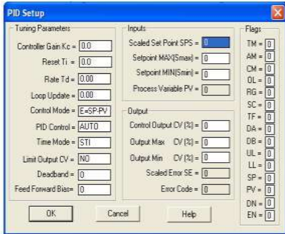
Fig. 3, PID Controller in SCADA
