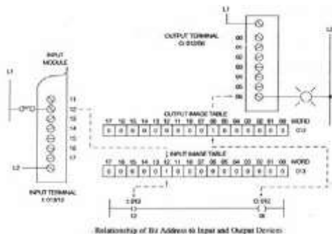
Fig. 1, I/O Pin Configuration of AB PLC
