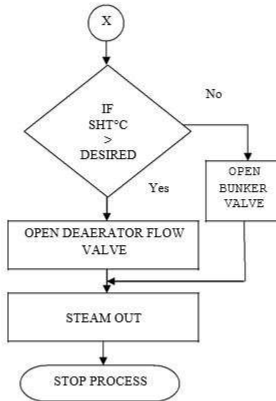
Fig.4, Flow chart of Boiler Operation
