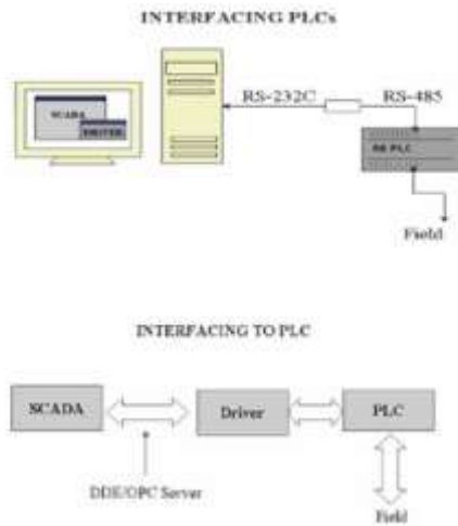
Fig. 2, Interfacing of PLC and SCADA
