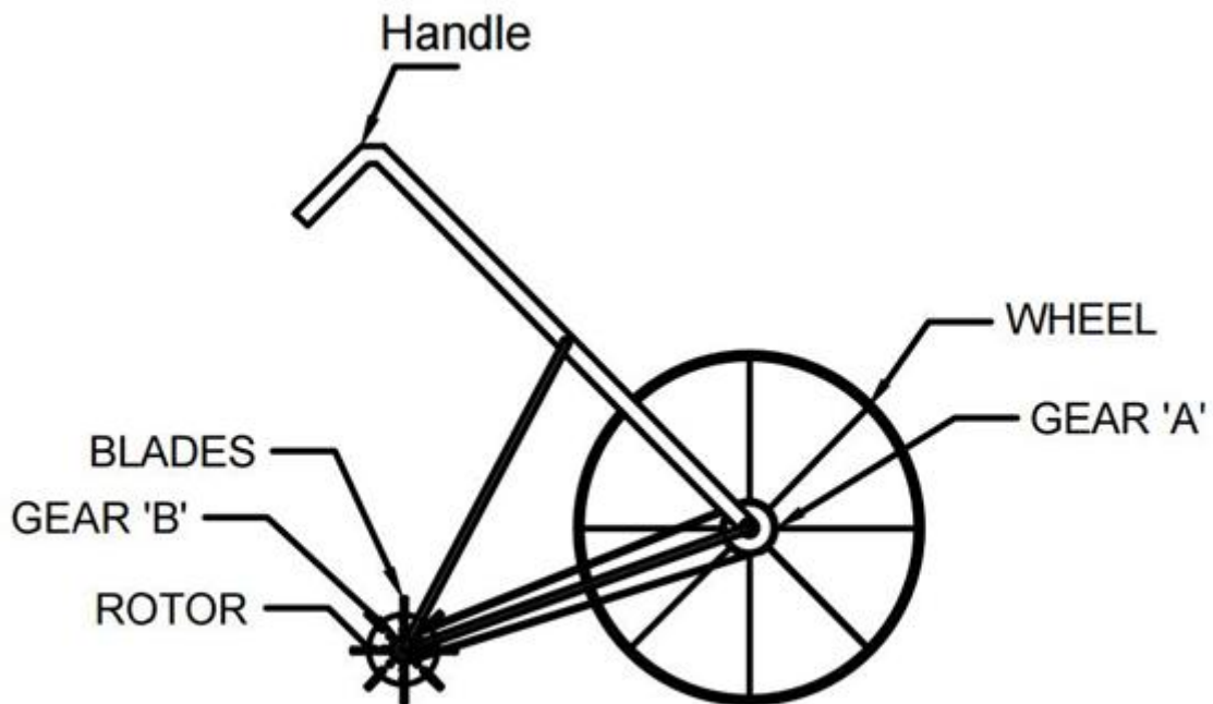
Fig. 1 Bicycle rotor
