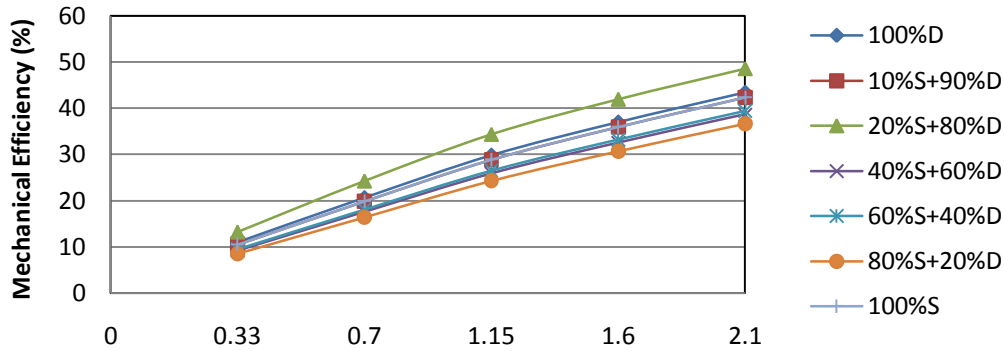
Graph No. 3 Comparison graph for mechanical efficiency
