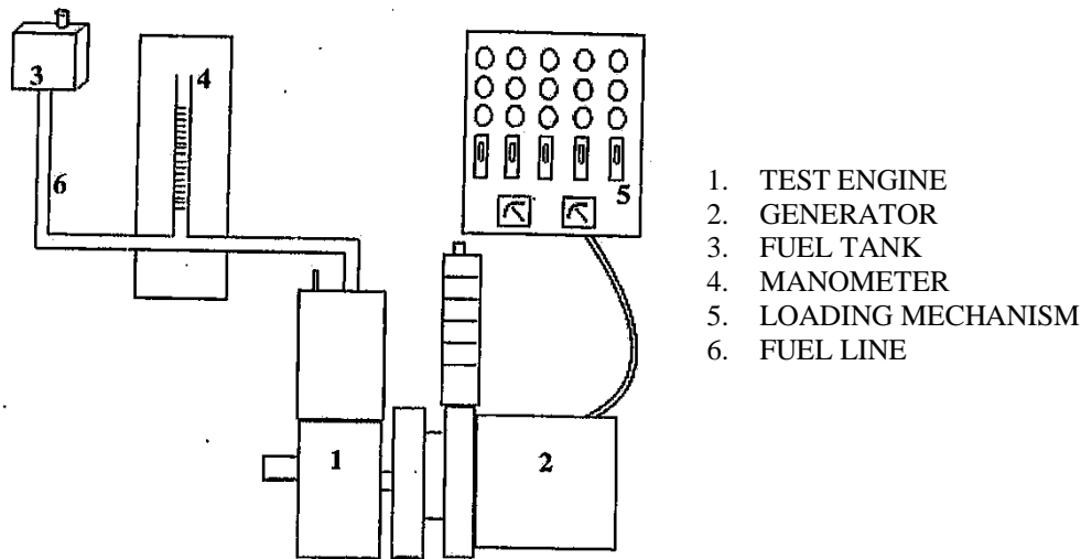
Fig.1. Experimental setup for engine test
