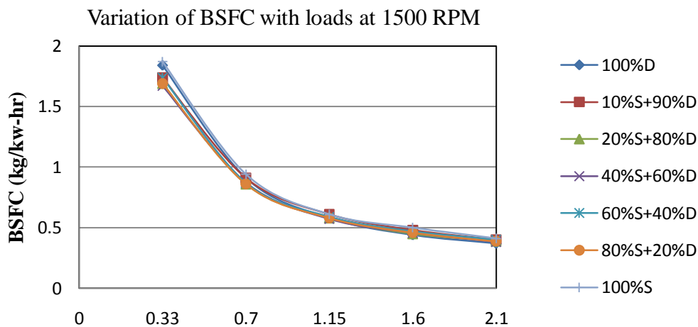
Graph No. 1 Comparison graph for BSFC
