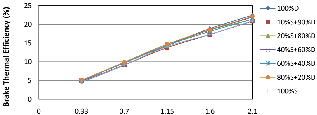
Graph No. 2 Comparison graph for thermal efficiency
