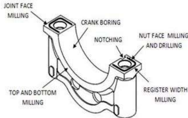
Figure 1: Bearing cap machining details
